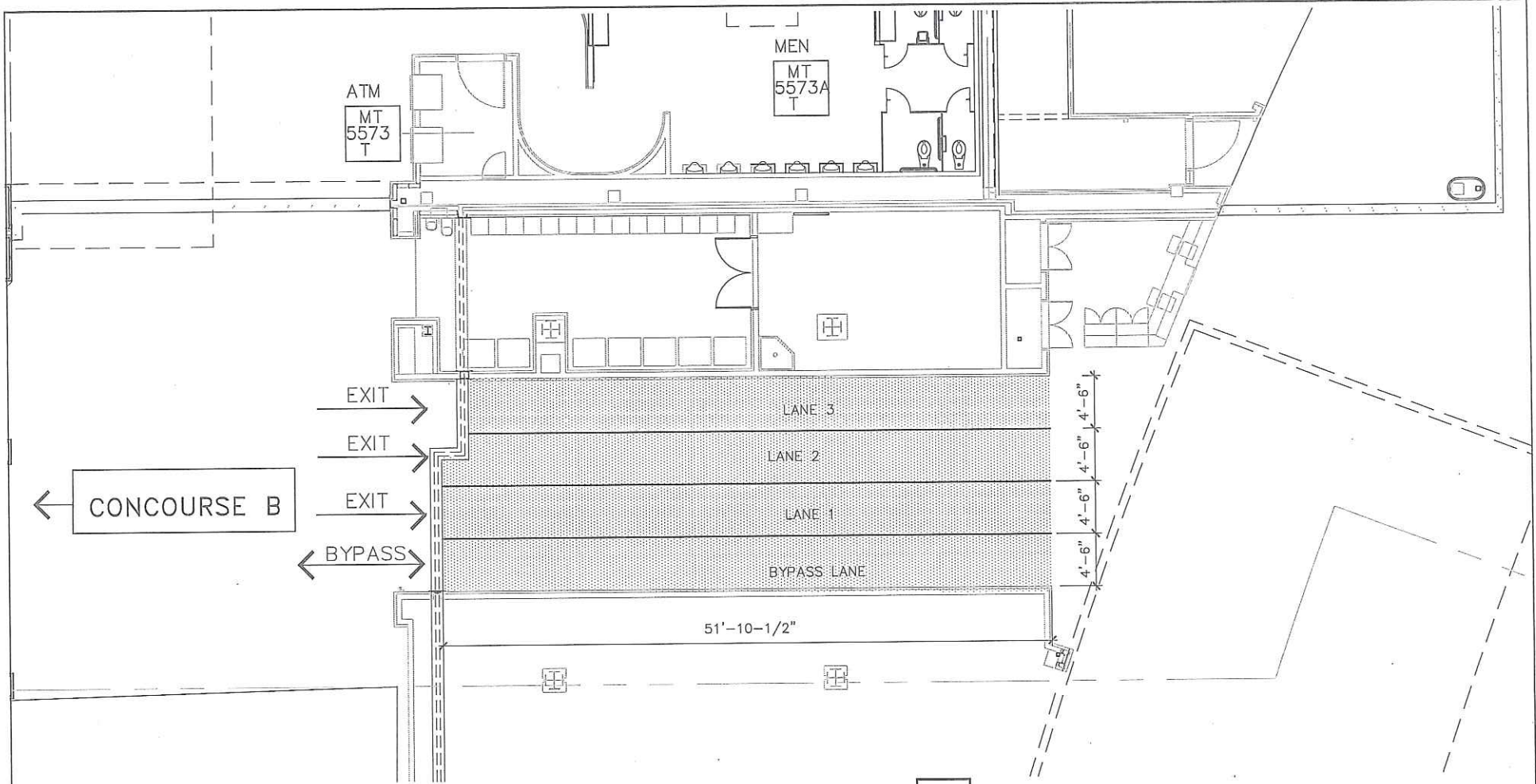
PLAN MAIN TERMINAL-EXIT B SCALE: 1/8" = 1'-0" 1 SK-02
